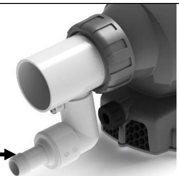
DIAGRAM 5 - INCORRECT EXTERNAL INSTALLATION
