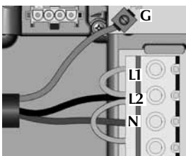
1-phase
