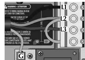
3-phases Delta
