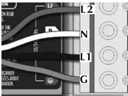
For 240 V (4 wires)
