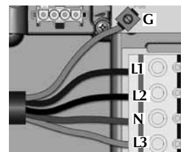
3-phases with single neutral
