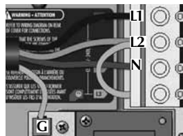
2-phases with single neutral
